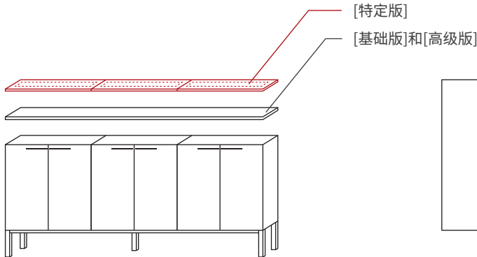
B W2400xD450xH1050mm
